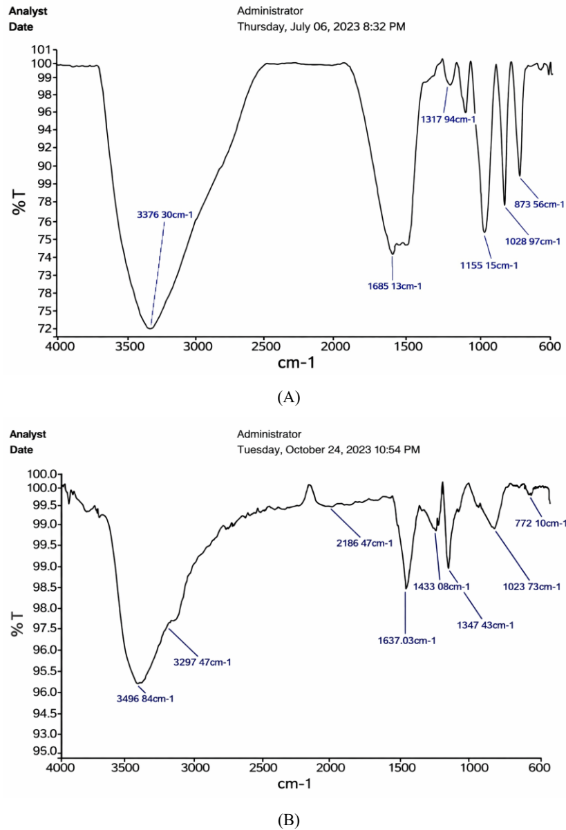
Figure 4. ATR-FTIR spectrum of (A) the raw sensor and (B) the sensor treated with ozone and UV.
