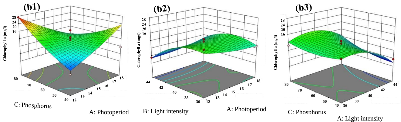
Figure 3: Presents a three-dimensional representation depicting the combined effects of varying light intensity levels, photoperiods, and different phosphorus concentrations on the efficiency of chlorophyll a in Chlorella vulgaris . In this figure, b1 represents the outcomes associated with the interaction of factors A and C, b2 corresponds to the results of the interaction between factors A and B, and b3 indicates the effects arising from the interaction of factors B and C.
